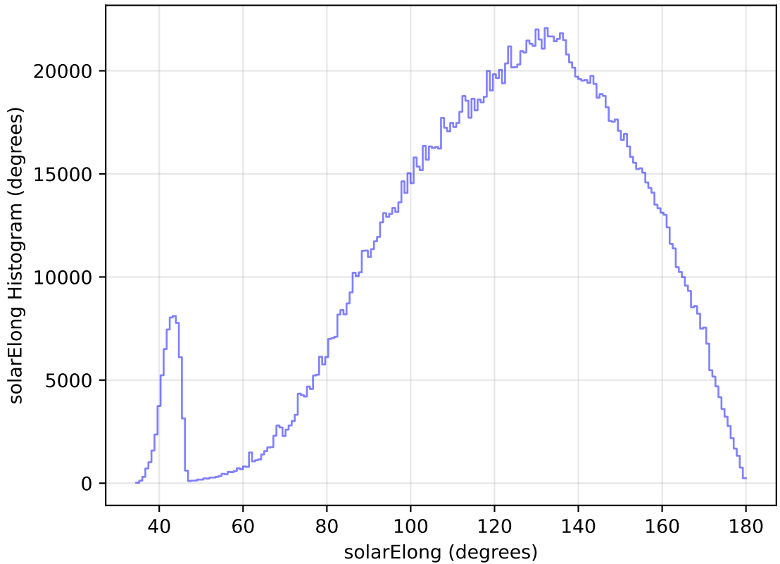
internal_u_expt27_nscale1.0v3.4_10yrs All sky all bands: solarElong Histogram
