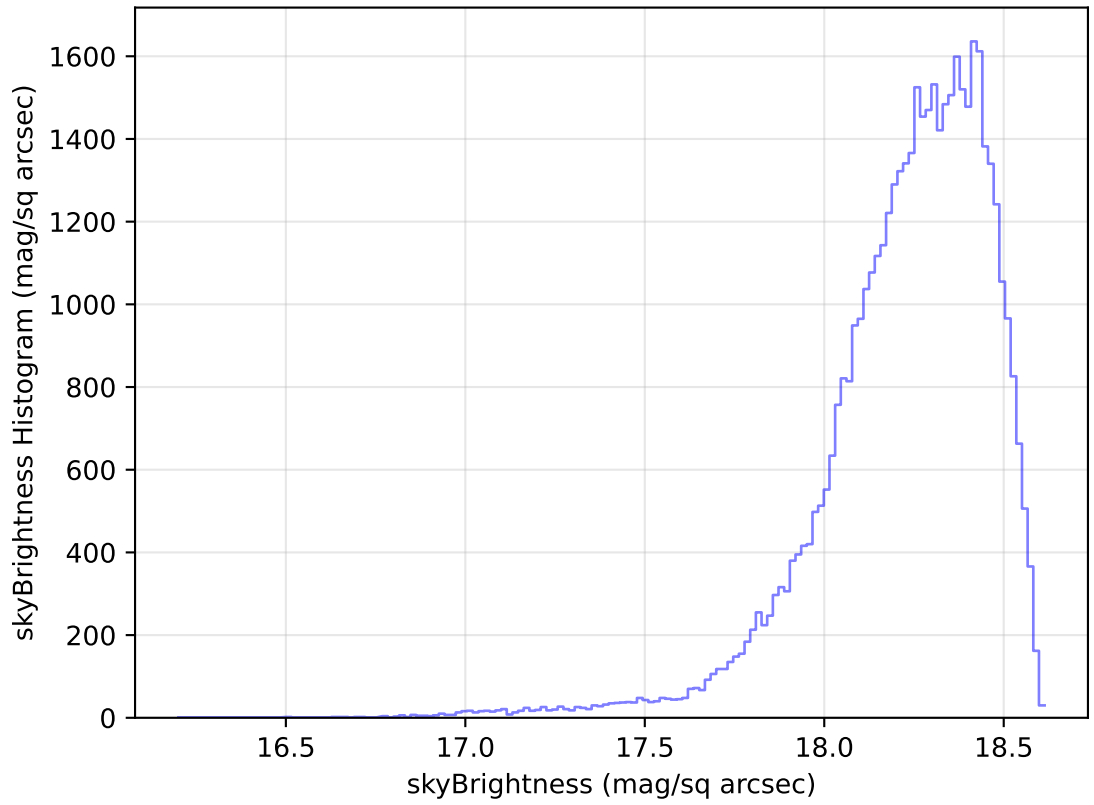
internal_u_expt27_nscale1.0v3.4_10yrs Yr 1 y band: skyBrightness Histogram
