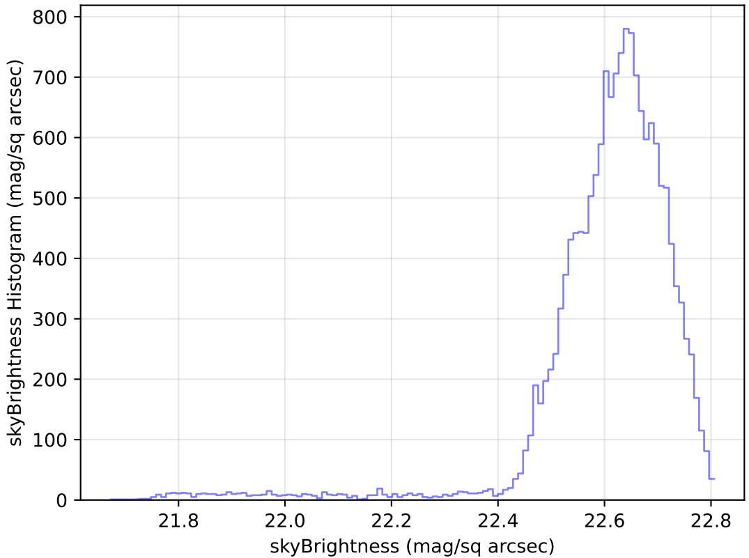
internal_u_expt27_nscale1.0v3.4_10yrs Yr 1 u band: skyBrightness Histogram
