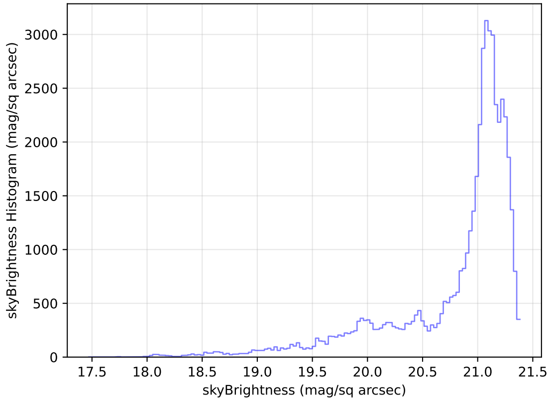
internal_u_expt27_nscale1.0v3.4_10yrs Yr 1 r band: skyBrightness Histogram
