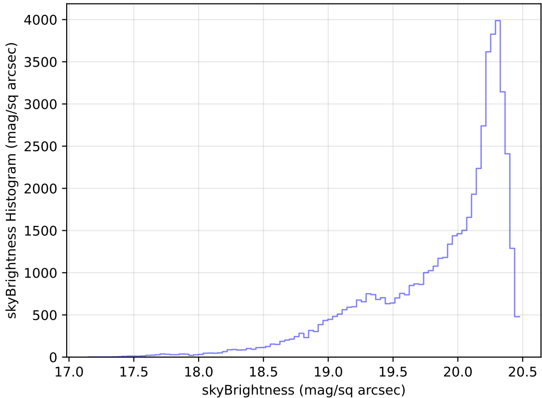
internal_u_expt27_nscale1.0v3.4_10yrs Yr 1 i band: skyBrightness Histogram
