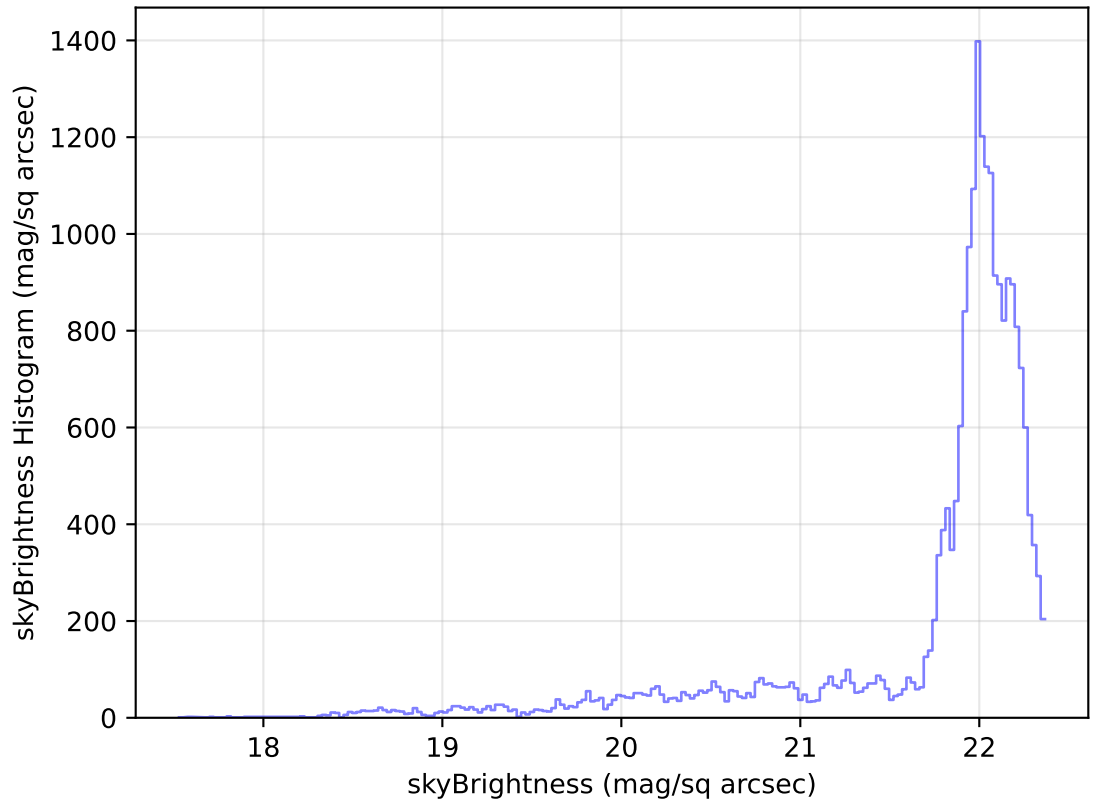
internal_u_expt27_nscale1.0v3.4_10yrs Yr 1 g band: skyBrightness Histogram
