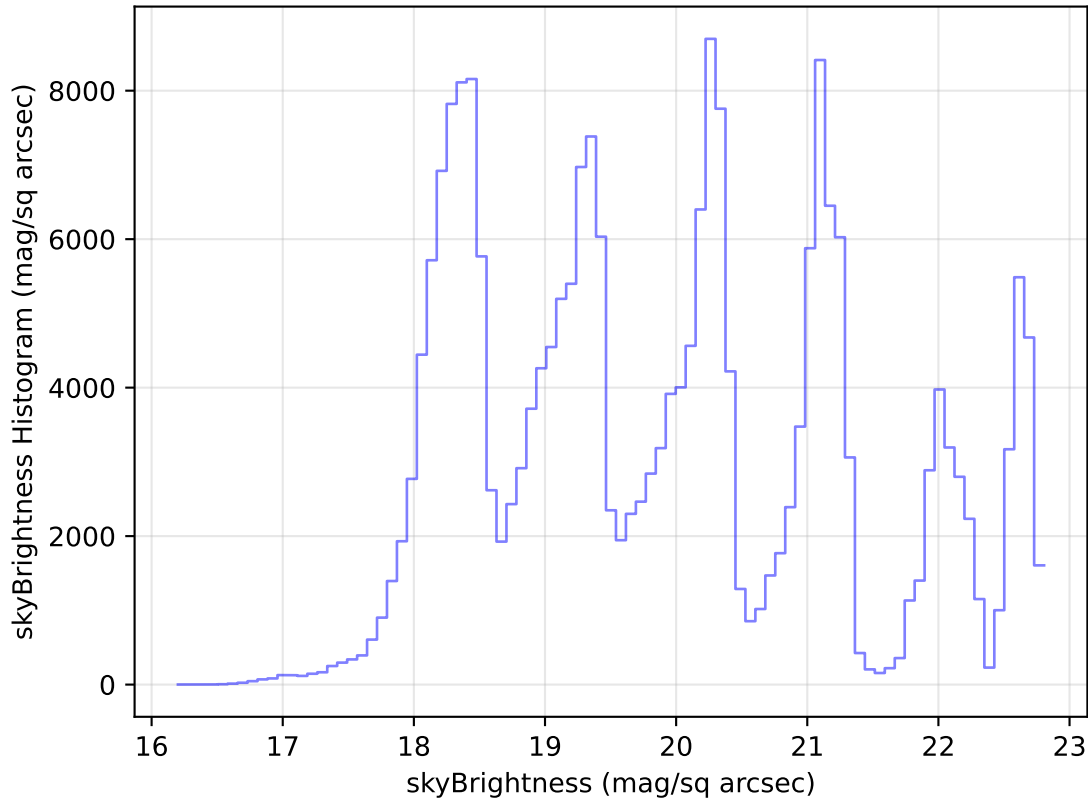
internal_u_expt27_nscale1.0v3.4_10yrs Yr 1 all bands: skyBrightness Histogram
