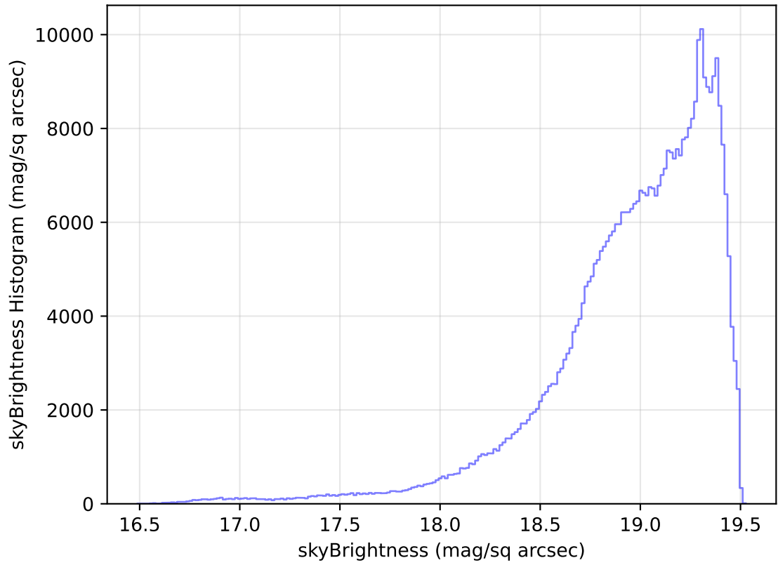
internal_u_expt27_nscale1.0v3.4_10yrs WFD z band: skyBrightness Histogram
