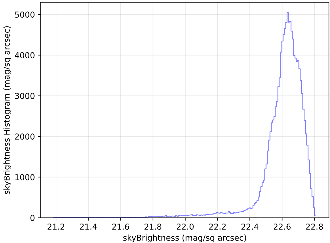
internal_u_expt27_nscale1.0v3.4_10yrs WFD u band: skyBrightness Histogram
