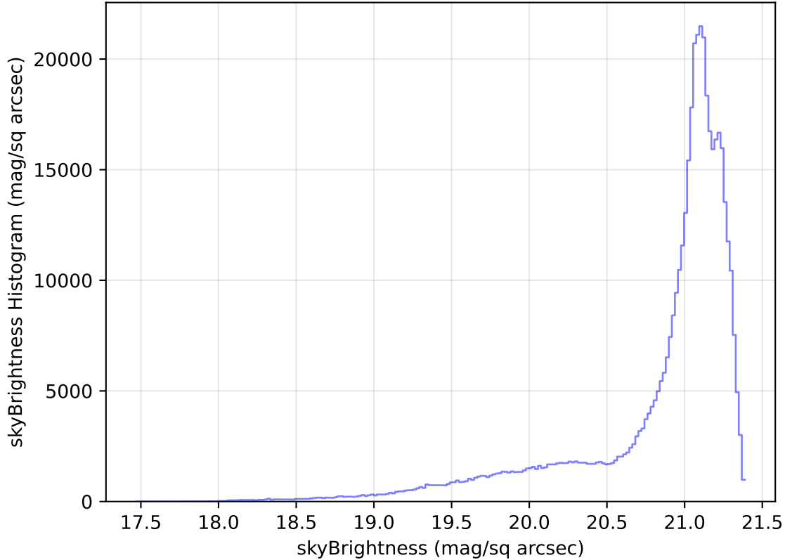
internal_u_expt27_nscale1.0v3.4_10yrs WFD r band: skyBrightness Histogram
