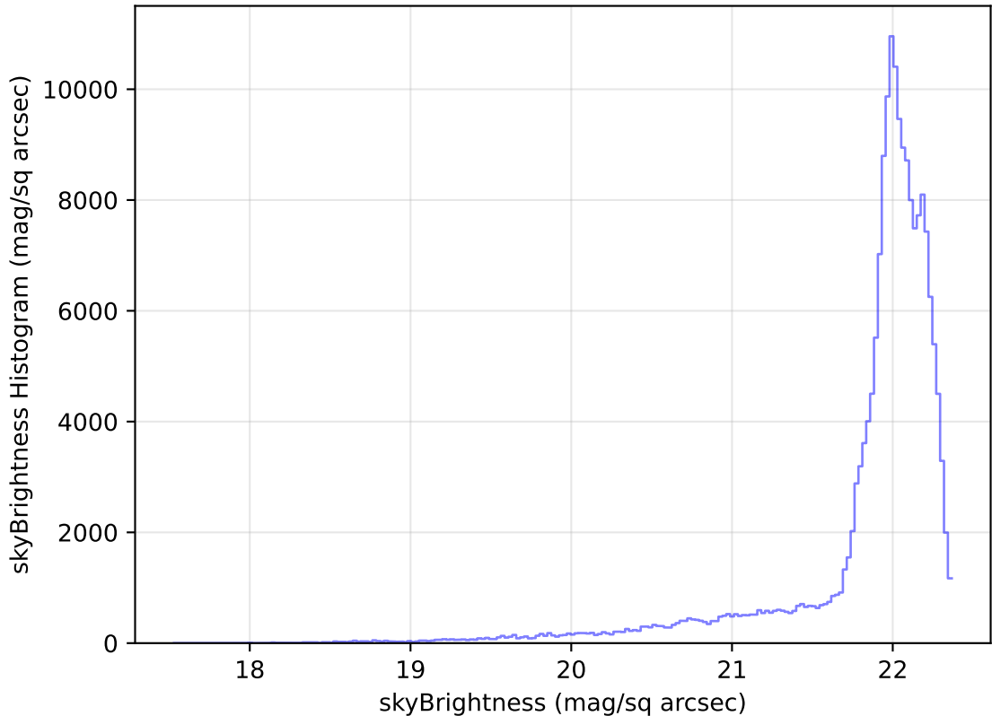
internal_u_expt27_nscale1.0v3.4_10yrs WFD g band: skyBrightness Histogram
