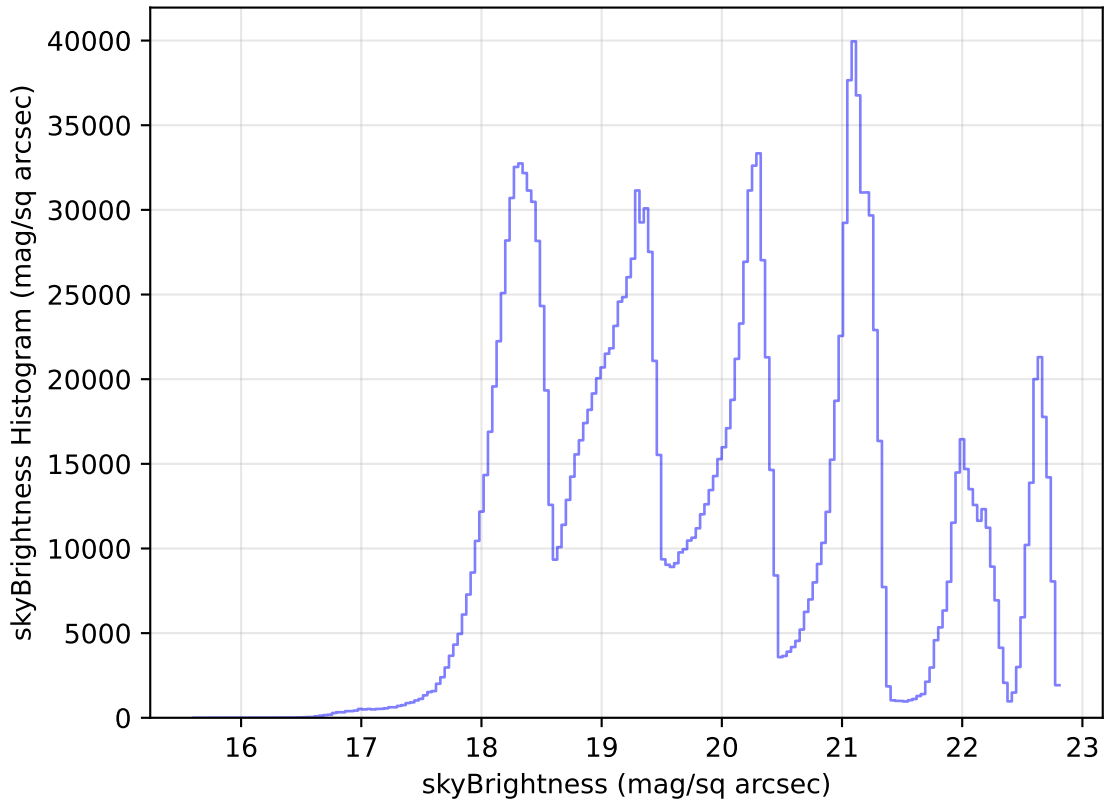
internal_u_expt27_nscale1.0v3.4_10yrs WFD all bands: skyBrightness Histogram
