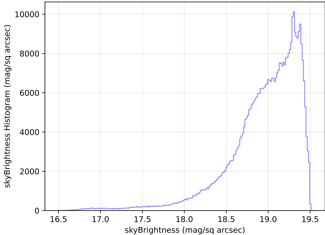
internal_u_expt27_nscale1.0v3.4_10yrs All sky z band: skyBrightness Histogram
