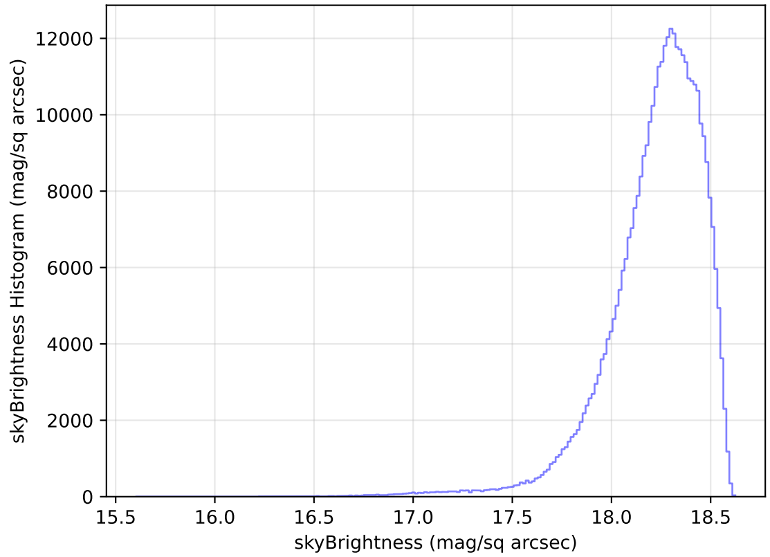
internal_u_expt27_nscale1.0v3.4_10yrs All sky y band: skyBrightness Histogram
