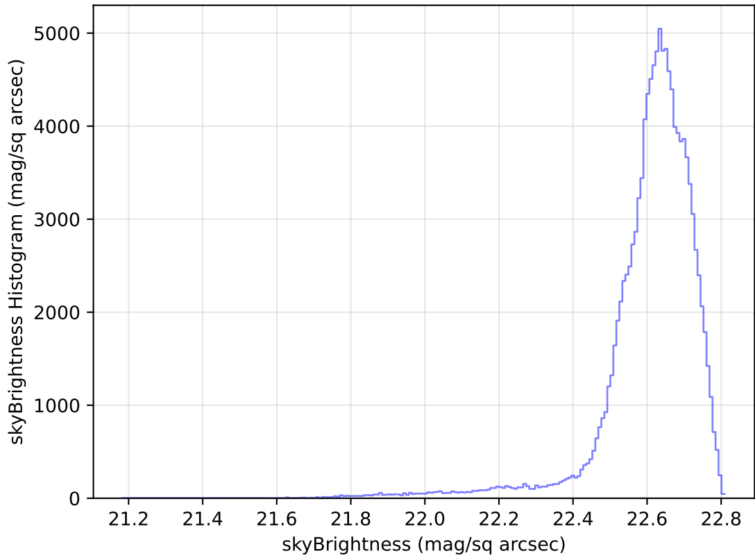
internal_u_expt27_nscale1.0v3.4_10yrs All sky u band: skyBrightness Histogram
