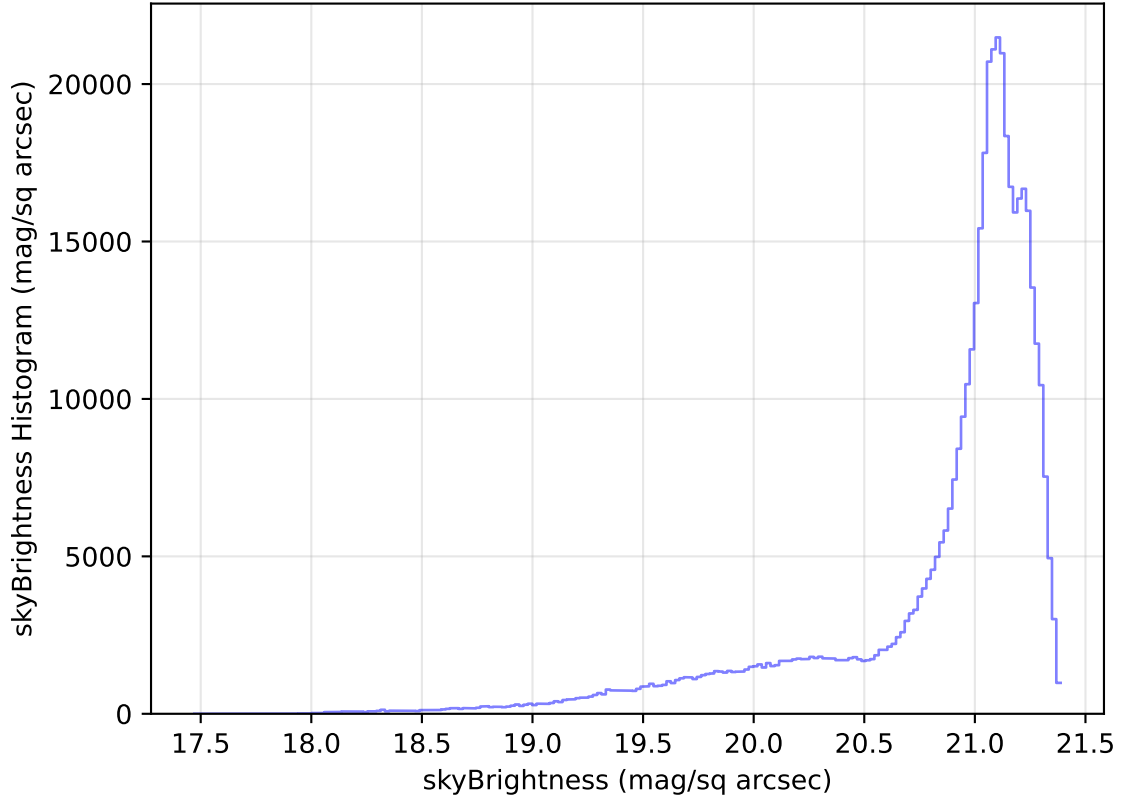
internal_u_expt27_nscale1.0v3.4_10yrs All sky r band: skyBrightness Histogram
