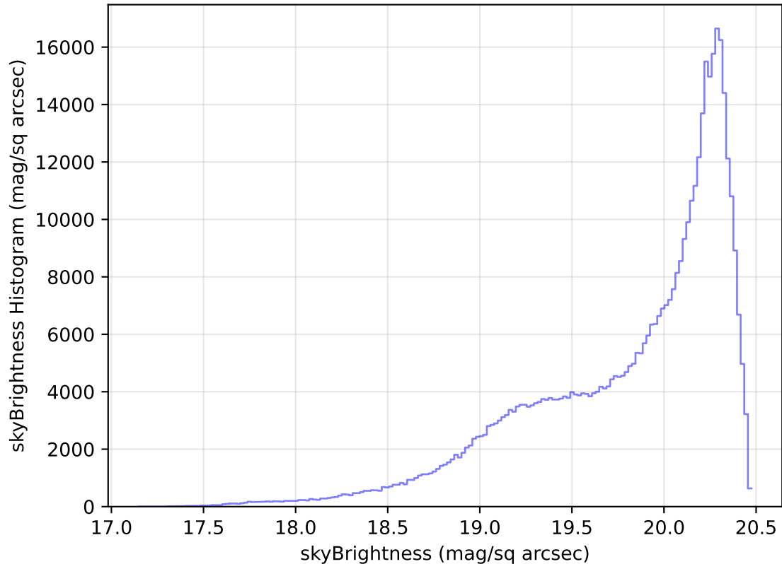
internal_u_expt27_nscale1.0v3.4_10yrs All sky i band: skyBrightness Histogram
