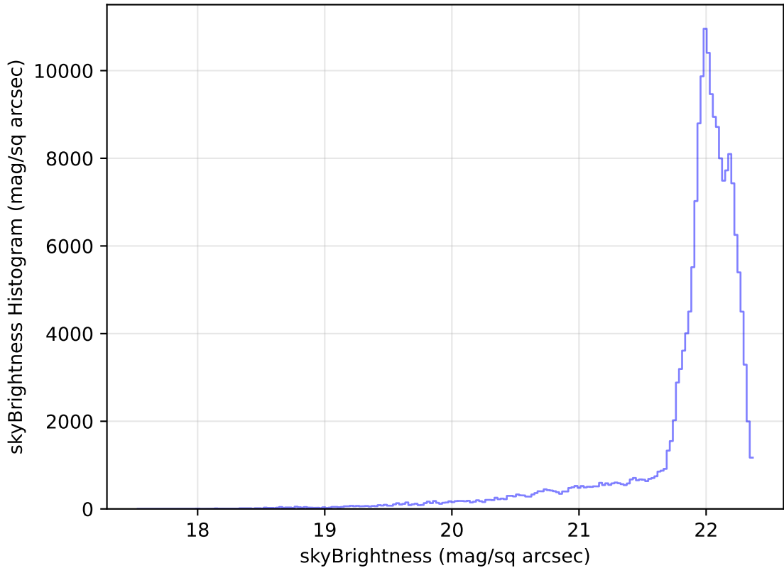
internal_u_expt27_nscale1.0v3.4_10yrs All sky g band: skyBrightness Histogram
