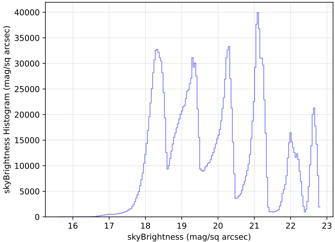
internal_u_expt27_nscale1.0v3.4_10yrs All sky all bands: skyBrightness Histogram
