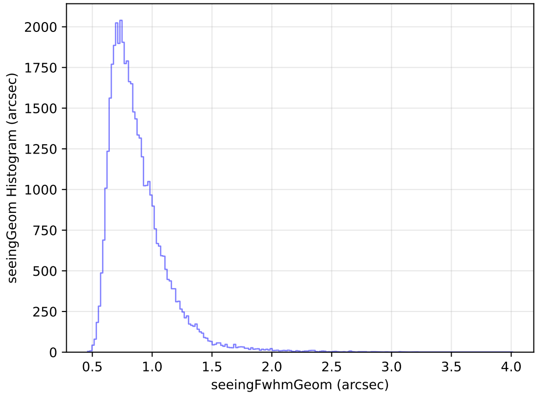
internal_u_expt27_nscale1.0v3.4_10yrs Yr 1 z band: seeingGeom Histogram
