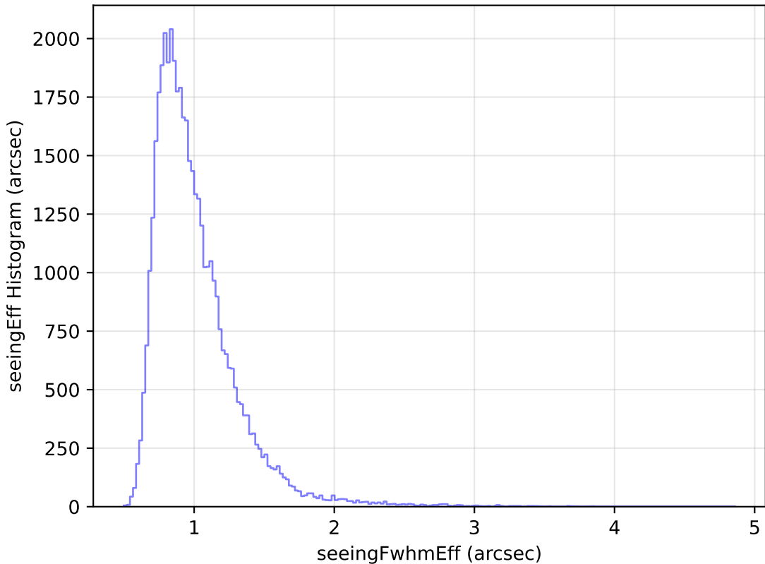
internal_u_expt27_nscale1.0v3.4_10yrs Yr 1 z band: seeingEff Histogram
