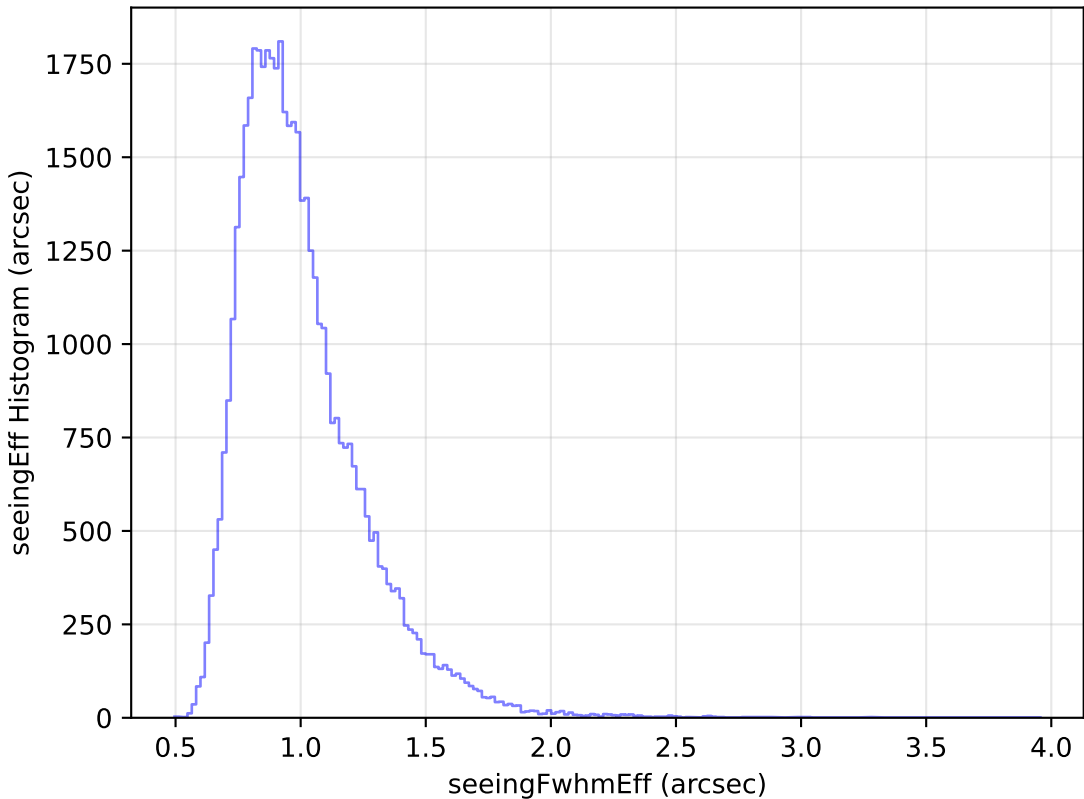
internal_u_expt27_nscale1.0v3.4_10yrs Yr 1 y band: seeingEff Histogram
