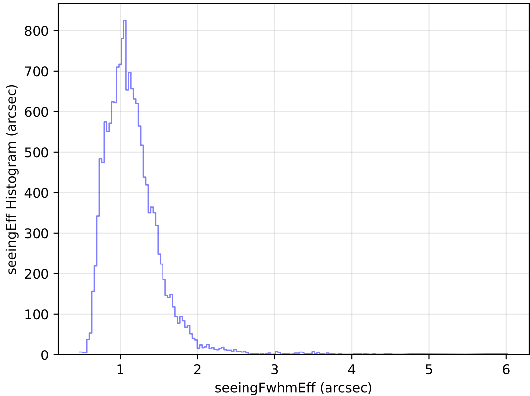
internal_u_expt27_nscale1.0v3.4_10yrs Yr 1 u band: seeingEff Histogram
