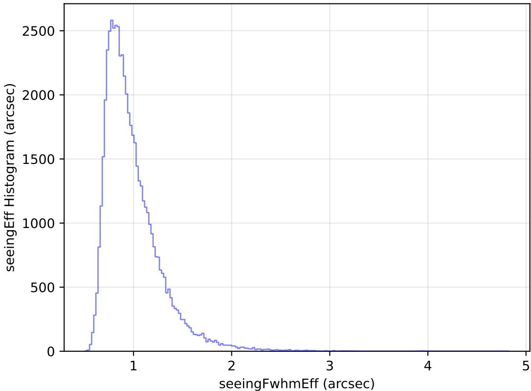
internal_u_expt27_nscale1.0v3.4_10yrs Yr 1 i band: seeingEff Histogram
