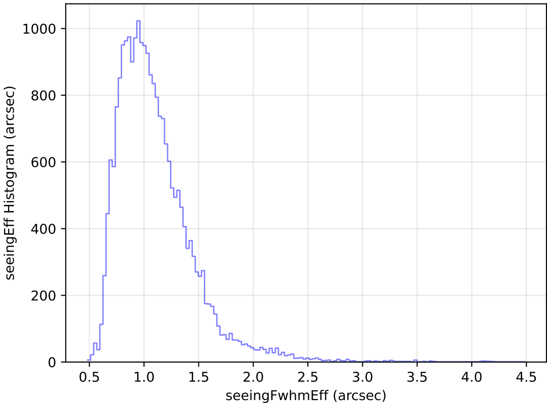
internal_u_expt27_nscale1.0v3.4_10yrs Yr 1 g band: seeingEff Histogram
