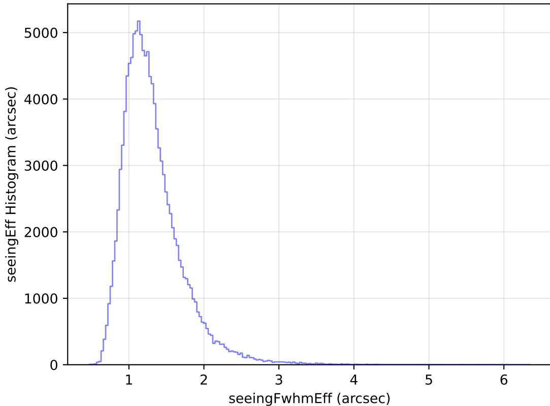
internal_u_expt27_nscale1.0v3.4_10yrs WFD u band: seeingEff Histogram
