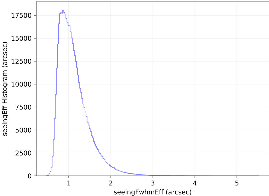
internal_u_expt27_nscale1.0v3.4_10yrs WFD r band: seeingEff Histogram
