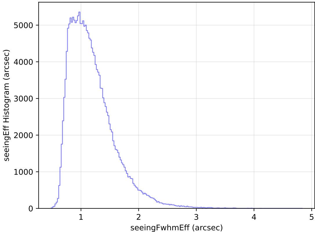
internal_u_expt27_nscale1.0v3.4_10yrs WFD g band: seeingEff Histogram
