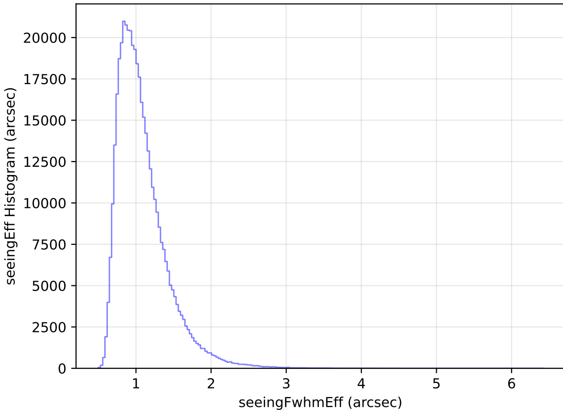
internal_u_expt27_nscale1.0v3.4_10yrs All sky z band: seeingEff Histogram
