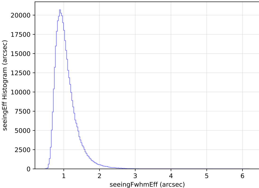
internal_u_expt27_nscale1.0v3.4_10yrs All sky y band: seeingEff Histogram
