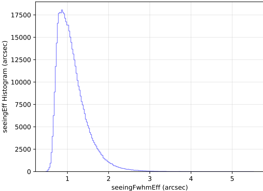
internal_u_expt27_nscale1.0v3.4_10yrs All sky r band: seeingEff Histogram
