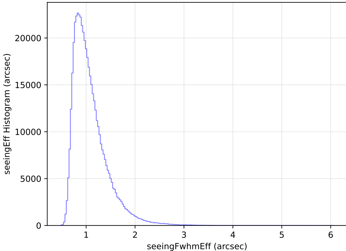
internal_u_expt27_nscale1.0v3.4_10yrs All sky i band: seeingEff Histogram
