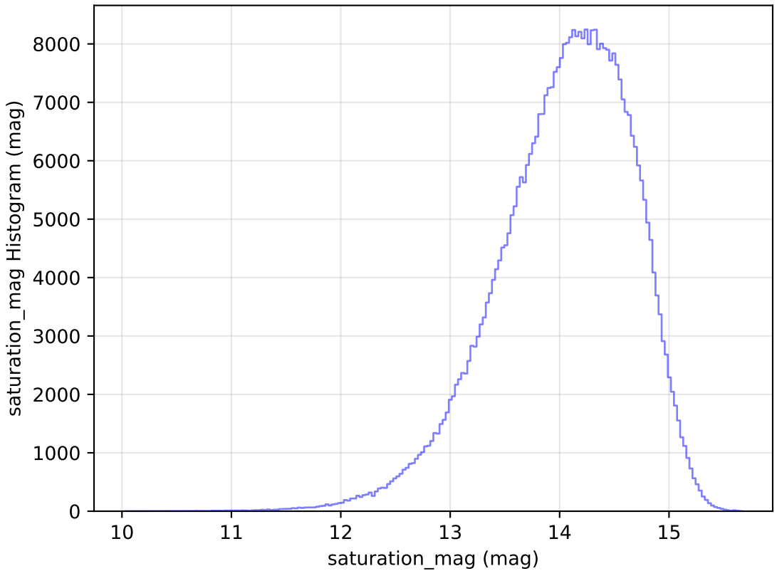
internal_u_expt27_nscale1.0v3.4_10yrs WFD z band: saturation_mag Histogram
