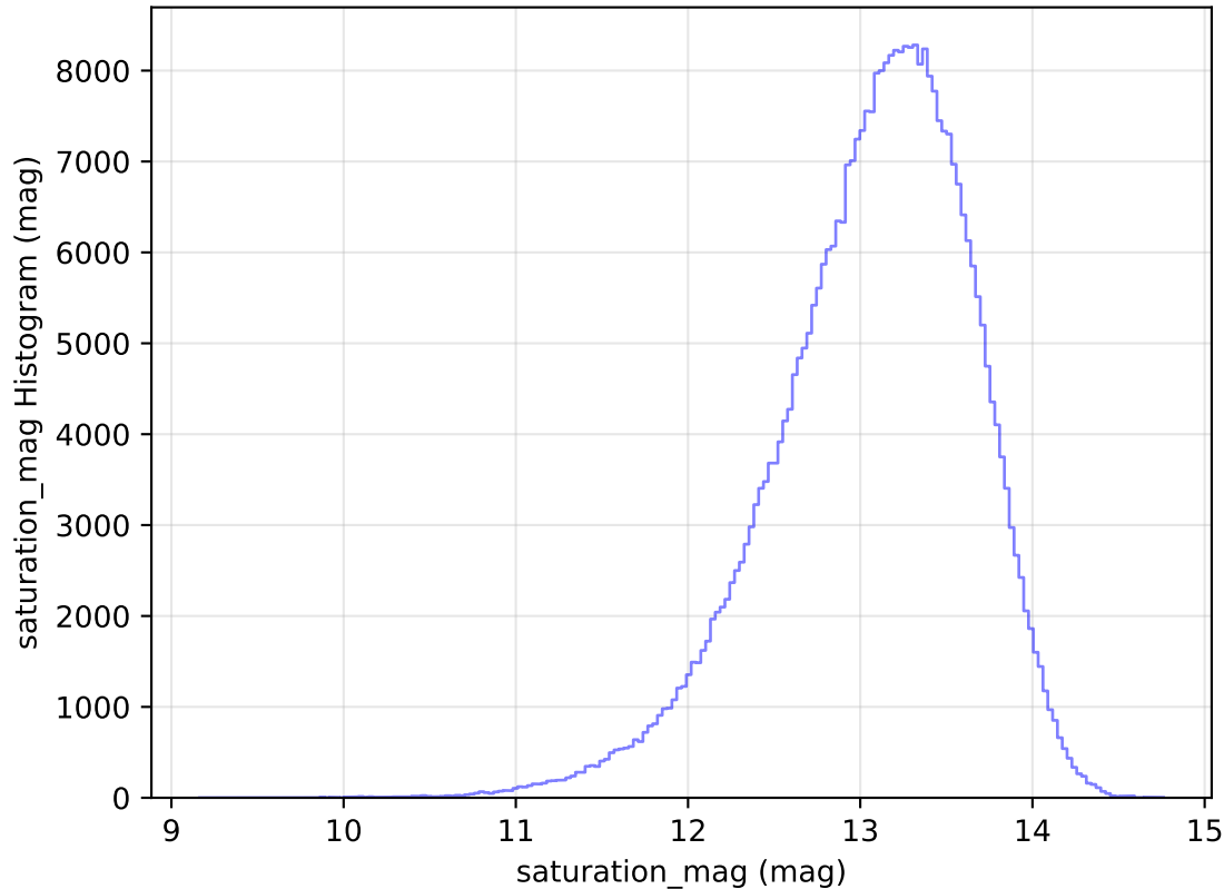
internal_u_expt27_nscale1.0v3.4_10yrs WFD y band: saturation_mag Histogram
