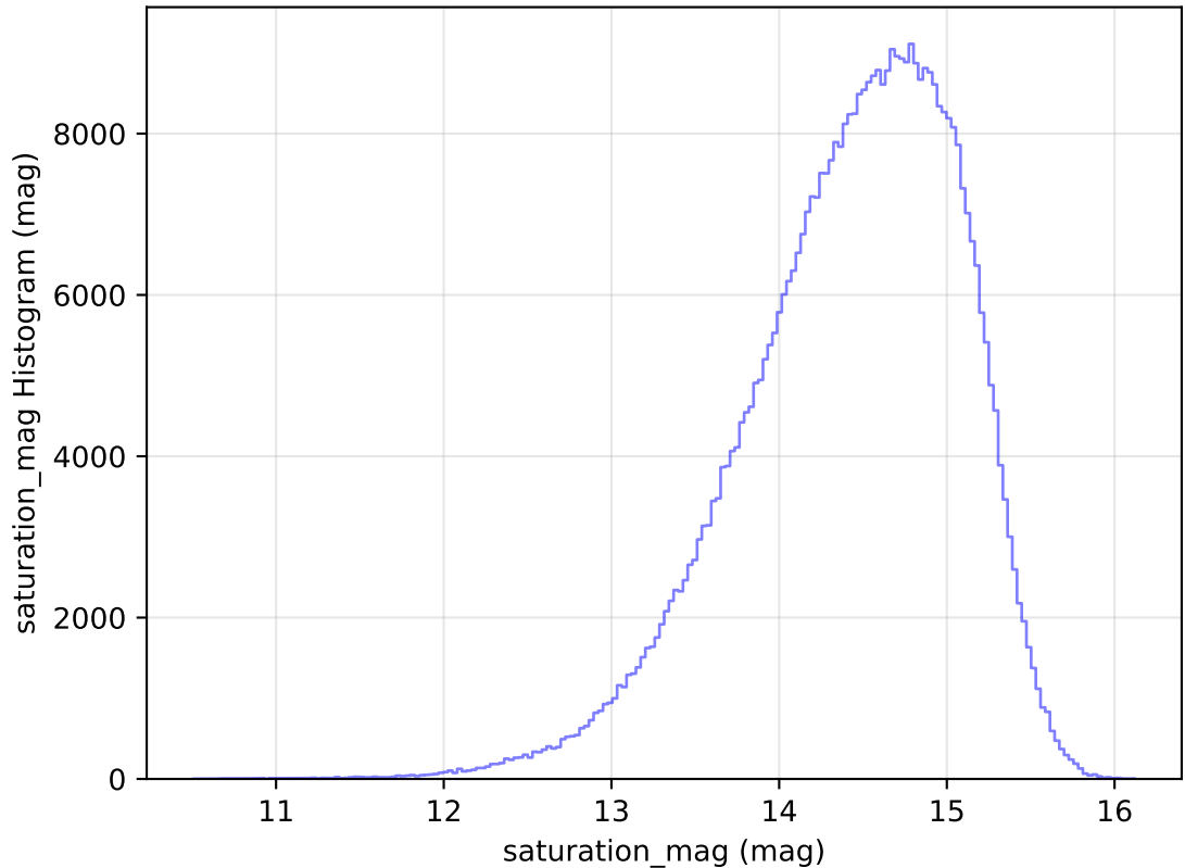
internal_u_expt27_nscale1.0v3.4_10yrs WFD i band: saturation_mag Histogram
