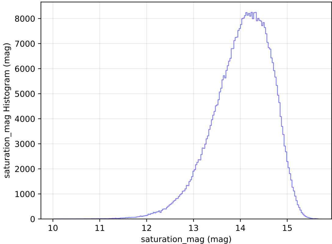
internal_u_expt27_nscale1.0v3.4_10yrs All sky z band: saturation_mag Histogram
