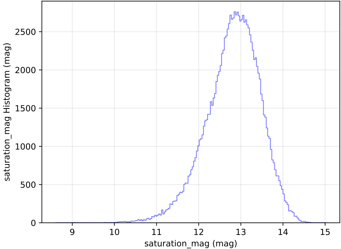
internal_u_expt27_nscale1.0v3.4_10yrs All sky u band: saturation_mag Histogram
