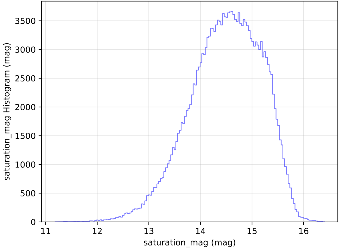
internal_u_expt27_nscale1.0v3.4_10yrs All sky g band: saturation_mag Histogram
