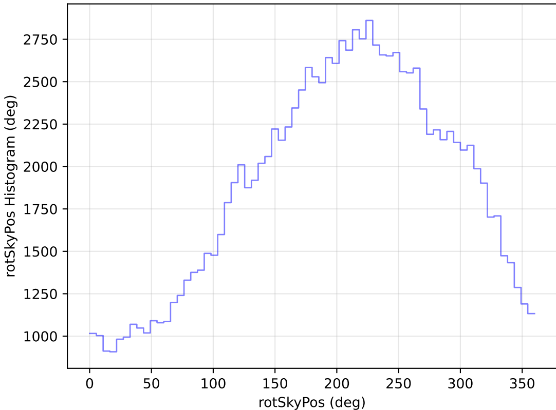
internal_u_expt27_nscale1.0v3.4_10yrs WFD u band: rotSkyPos Histogram
