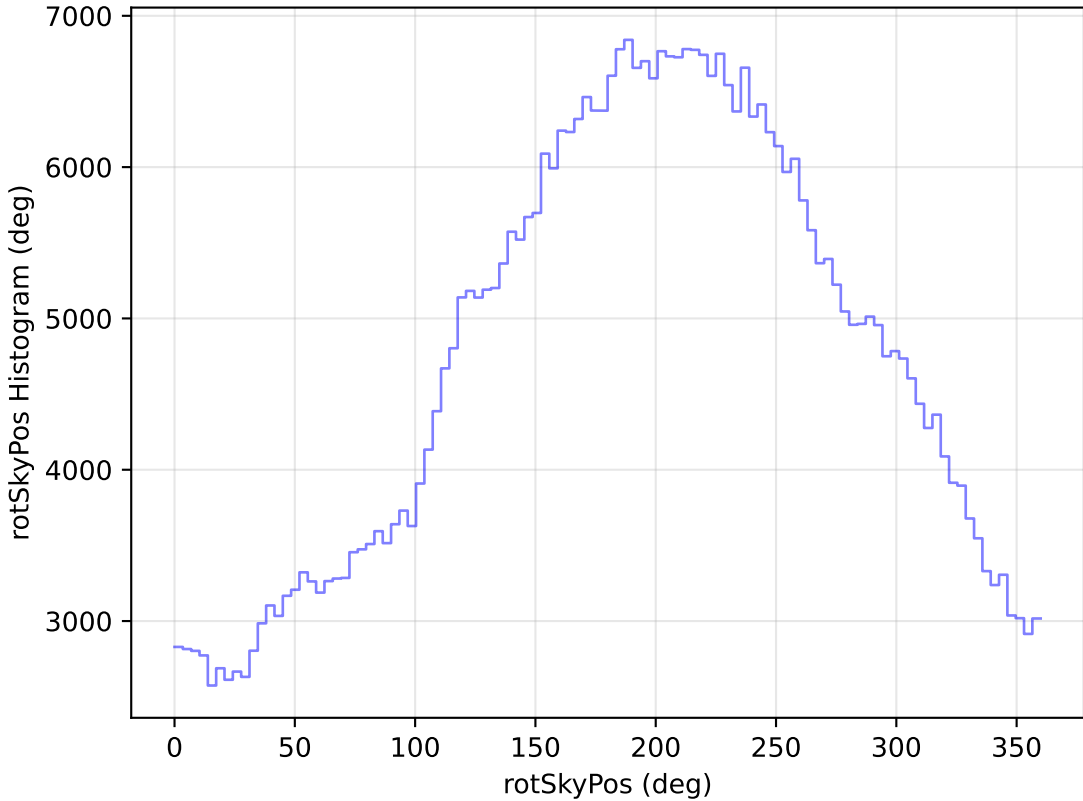
internal_u_expt27_nscale1.0v3.4_10yrs WFD r band: rotSkyPos Histogram
