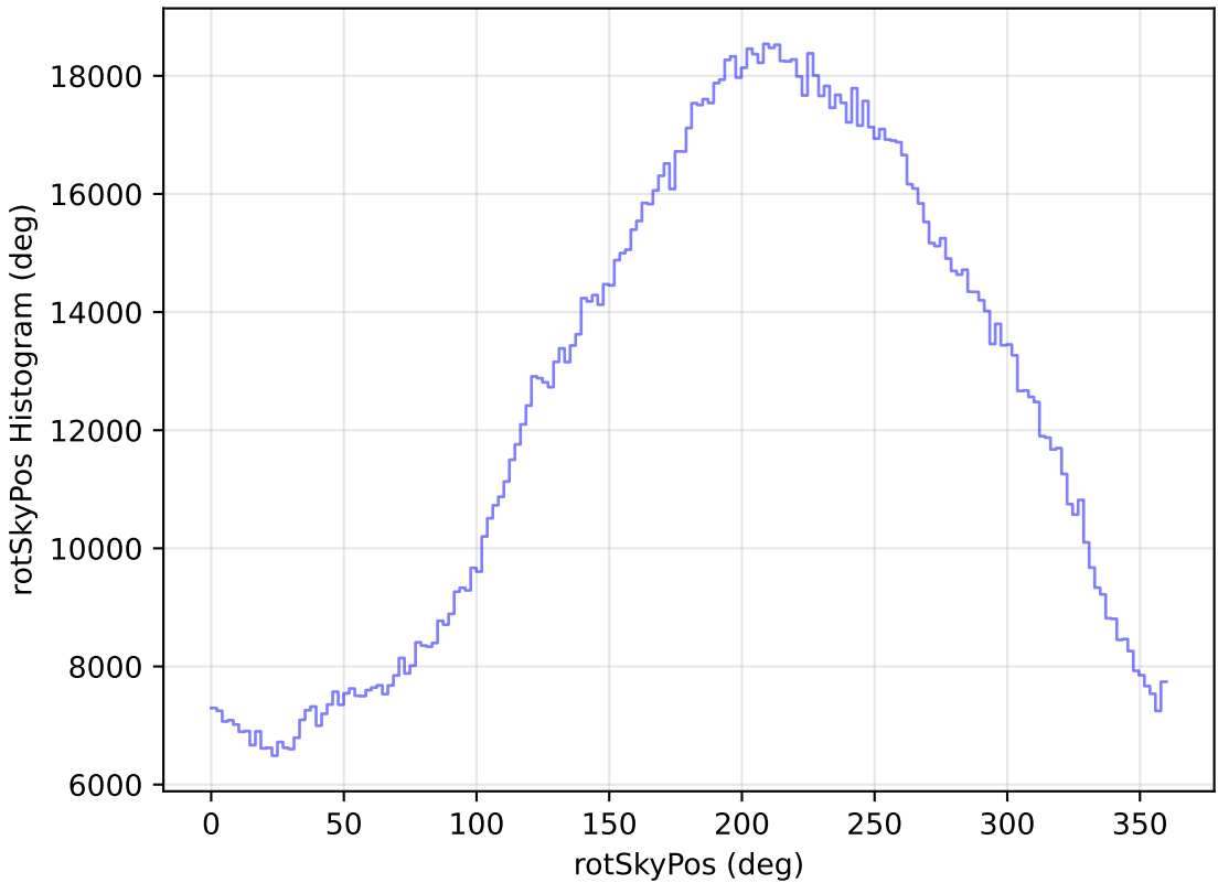
internal_u_expt27_nscale1.0v3.4_10yrs WFD all bands: rotSkyPos Histogram
