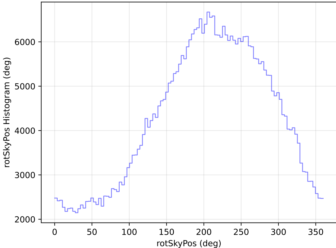
internal_u_expt27_nscale1.0v3.4_10yrs All sky z band: rotSkyPos Histogram
