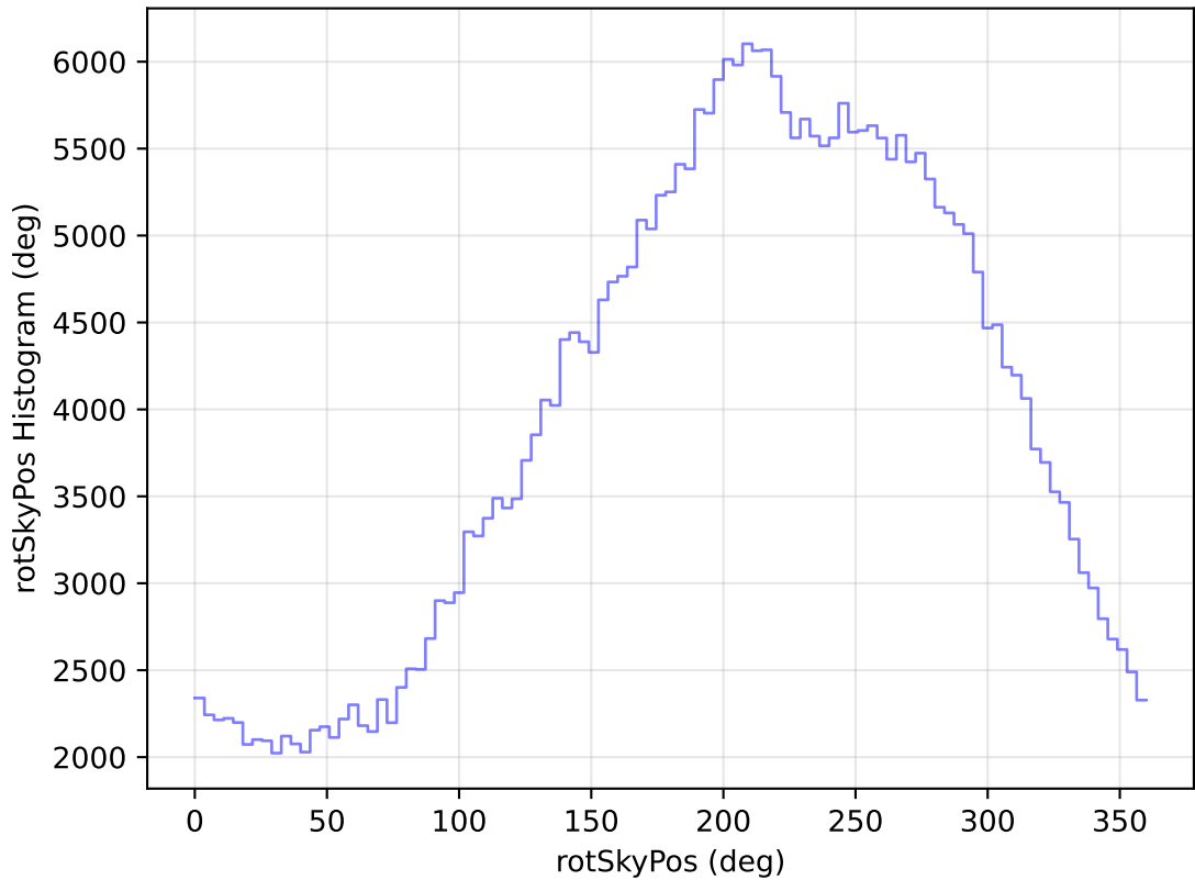
internal_u_expt27_nscale1.0v3.4_10yrs All sky y band: rotSkyPos Histogram
