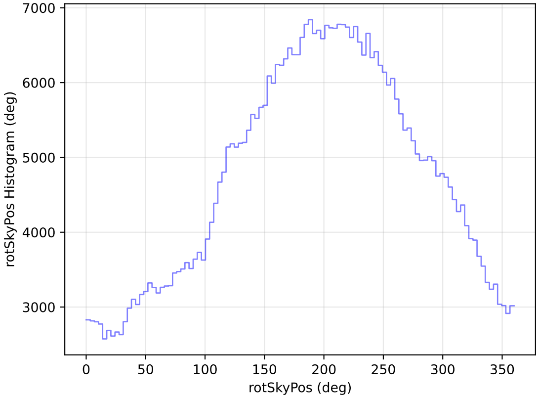
internal_u_expt27_nscale1.0v3.4_10yrs All sky r band: rotSkyPos Histogram
