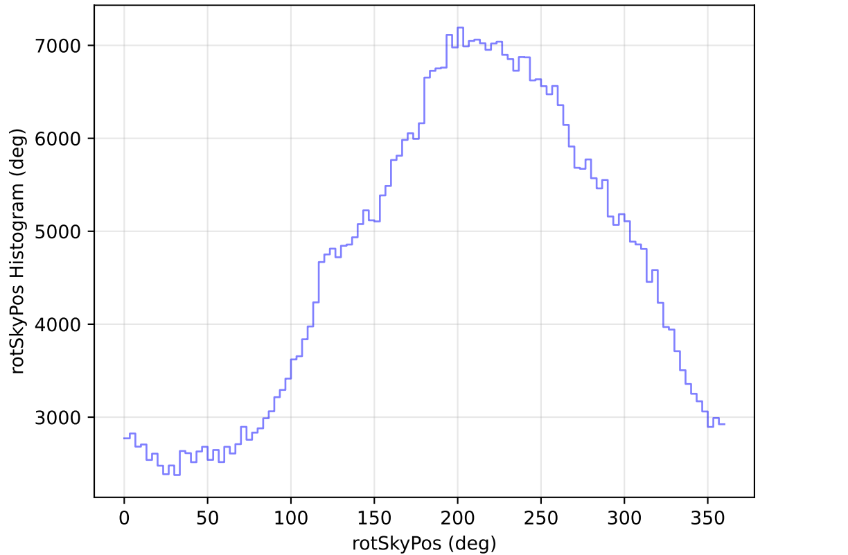
internal_u_expt27_nscale1.0v3.4_10yrs All sky i band: rotSkyPos Histogram
