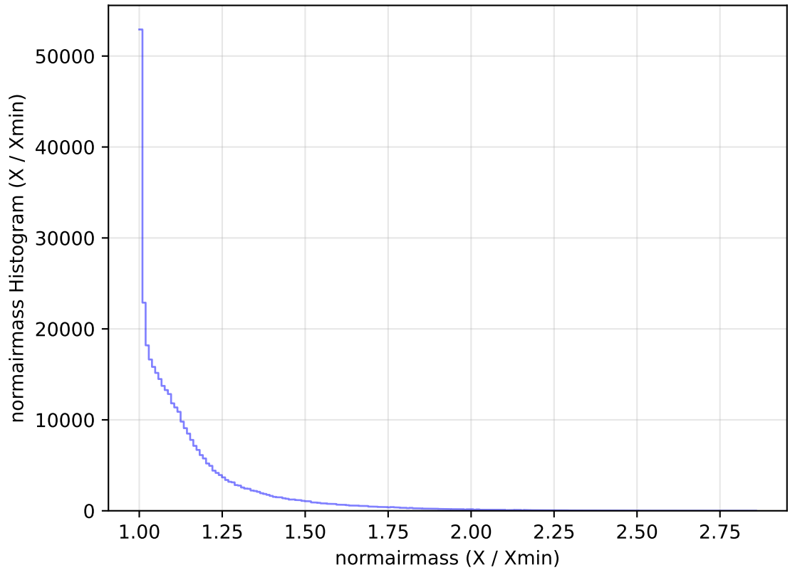
internal_u_expt27_nscale1.0v3.4_10yrs WFD y band: normairmass Histogram
