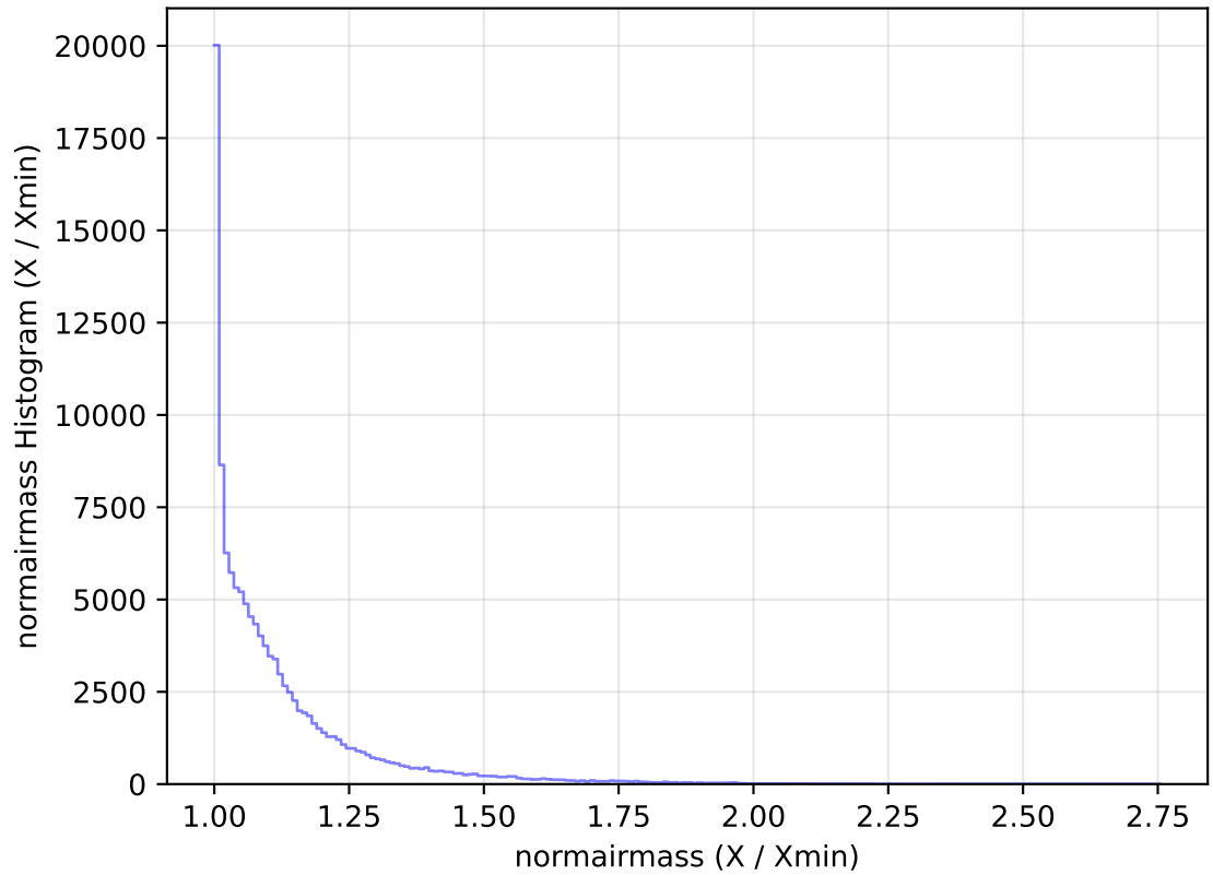
internal_u_expt27_nscale1.0v3.4_10yrs WFD u band: normairmass Histogram
