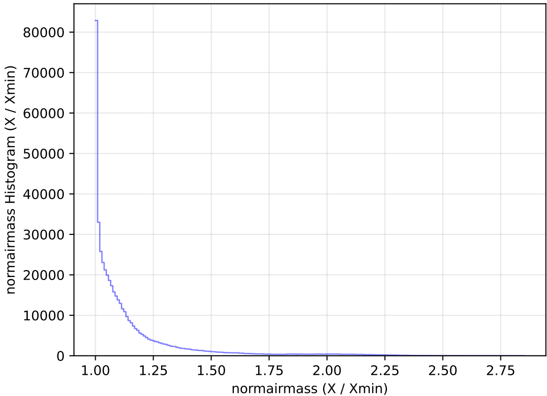
internal_u_expt27_nscale1.0v3.4_10yrs WFD r band: normairmass Histogram
