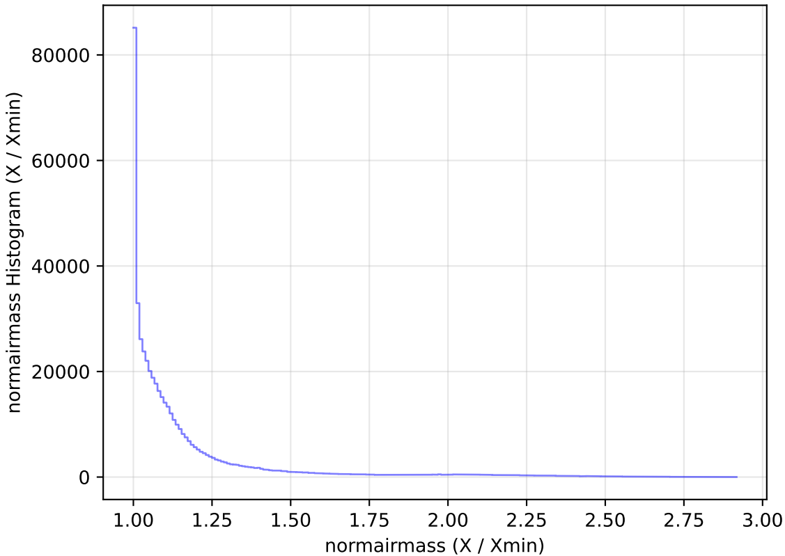
internal_u_expt27_nscale1.0v3.4_10yrs WFD i band: normairmass Histogram
