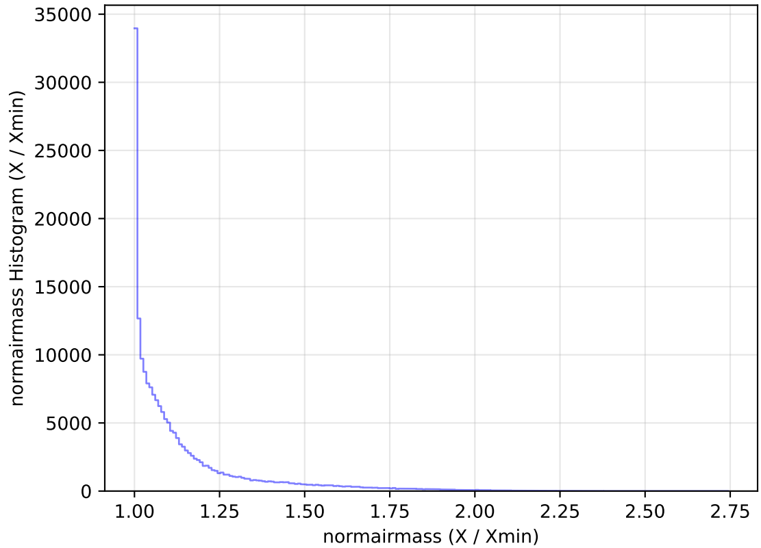
internal_u_expt27_nscale1.0v3.4_10yrs WFD g band: normairmass Histogram
